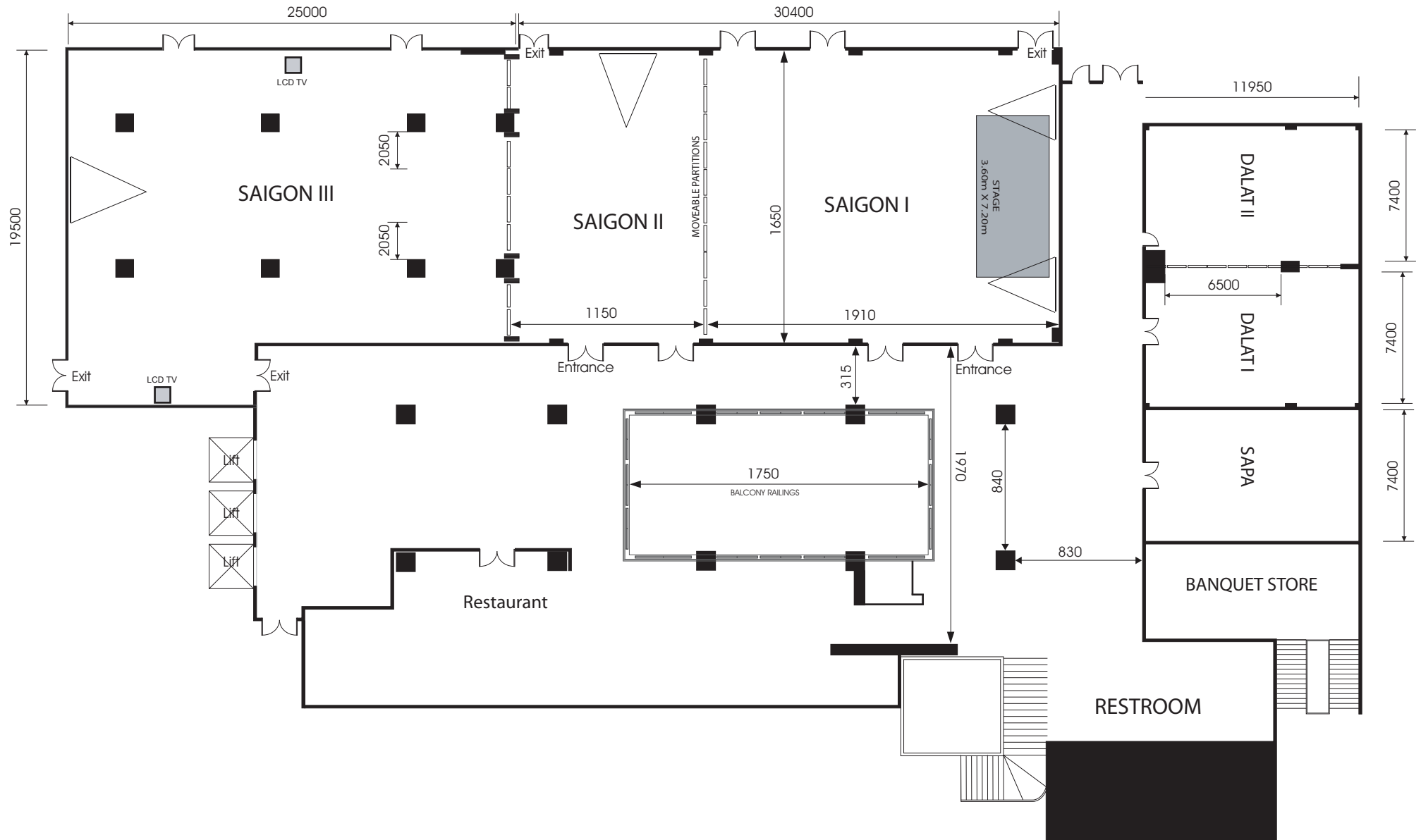
Hotel Equatorial HCMC The second Floor Layout
